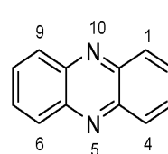
Phenazin
