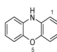
Phenoxazin
