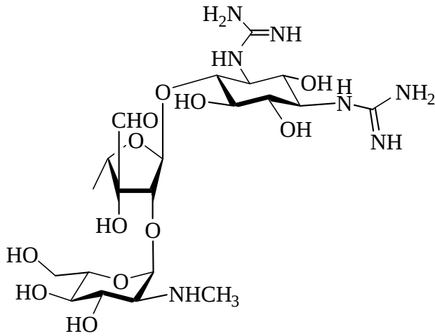
Streptomycin
