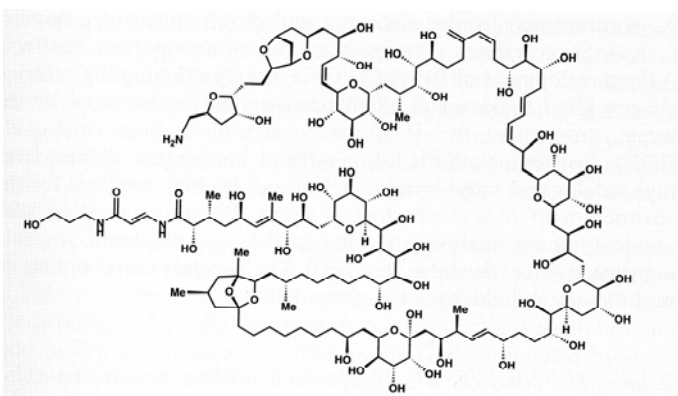
Palytoxin
