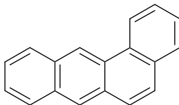
Tetraphen farblos
