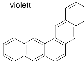
Pentaphen gelb
