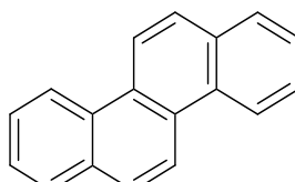
Chrysen
