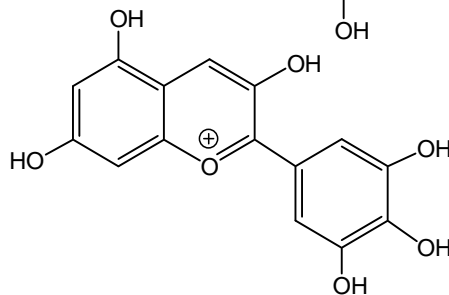
Delphinidin (violett)
