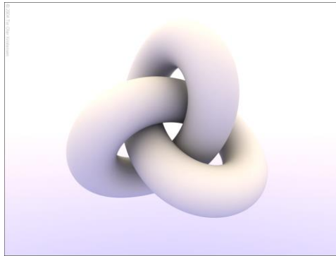
Trifoil (chiral)
